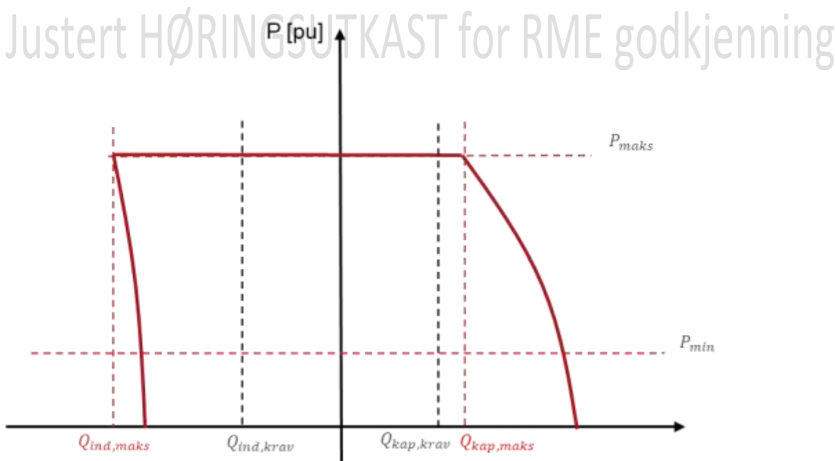
FIGUR 14-7: DRIFSDIAGRAM FOR EN KRAFTPARK REFERERT PCC.
