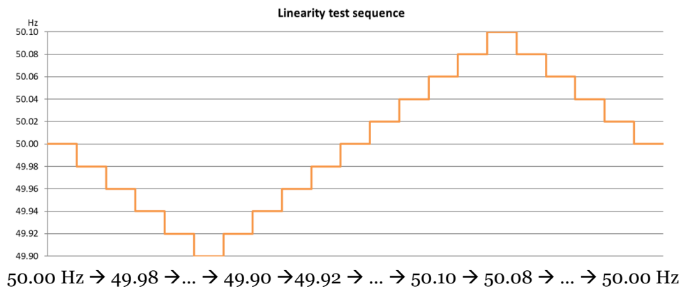
Figure 3. Linearity test sequence for FCR-N.
